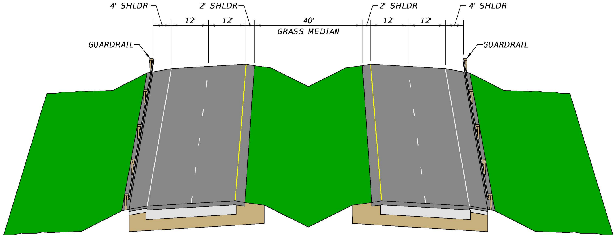
Existing Typical Section 1: Rural Mainline
