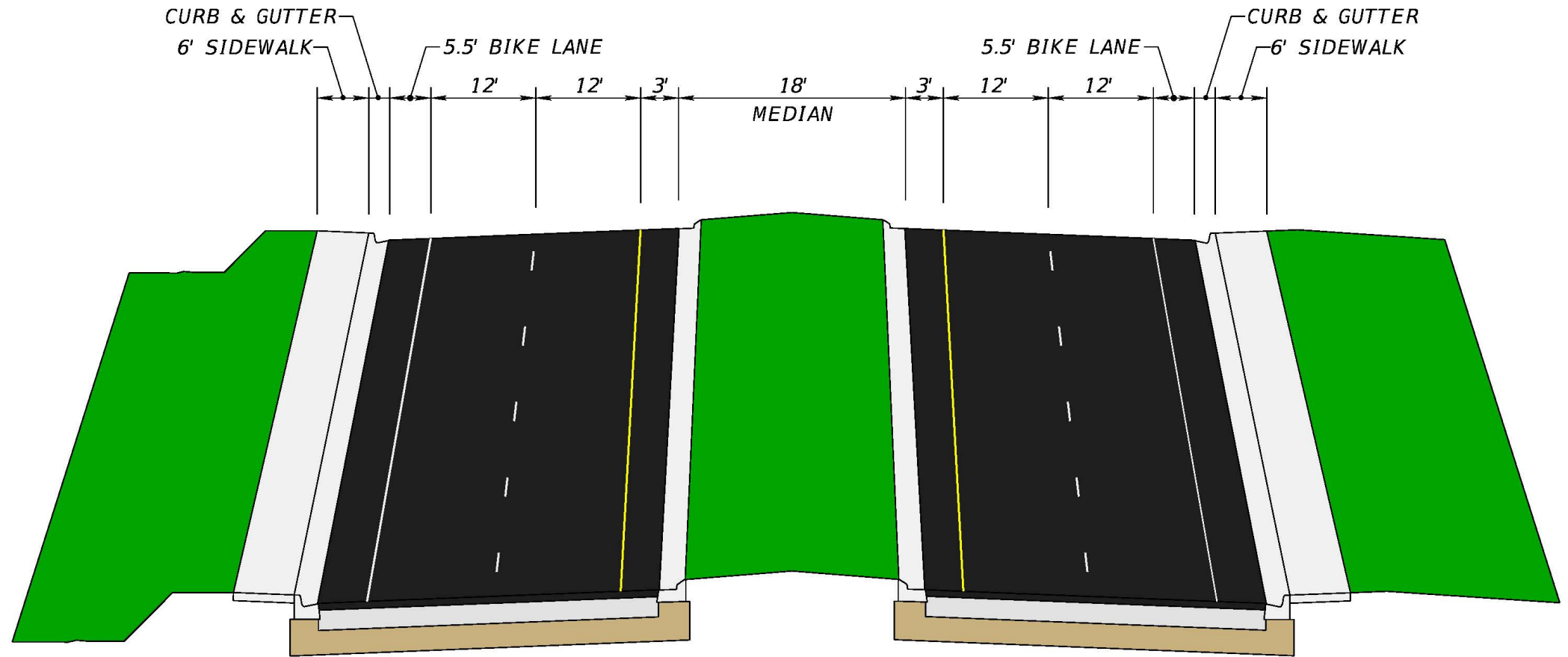
Proposed Typical Section 2: Urban Mainline
